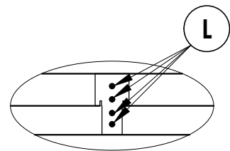
SECTION A-A (TYP. AT HEAD AND SILL)
